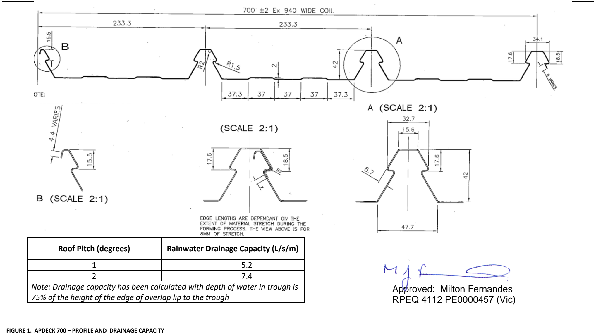
FIGURE 1. APDECK 700 – PROFILE AND DRAINAGE CAPACITY
